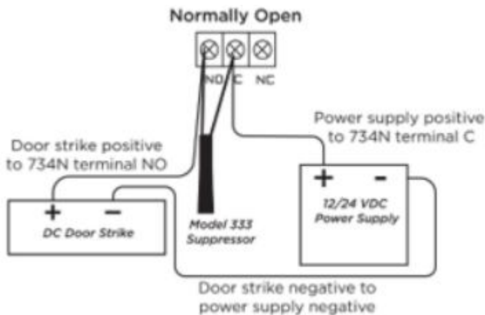
Typical Door Strike Wiring
