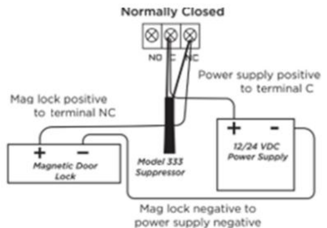
Typical Magnetic Lock Wiring
